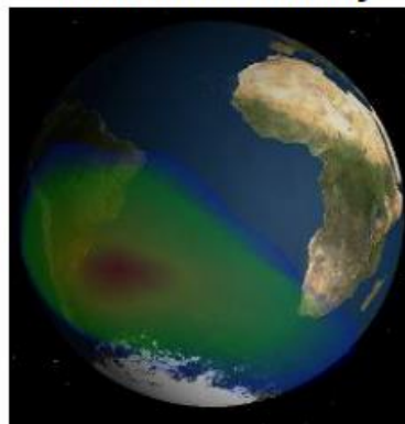
South atlantic anomaly
