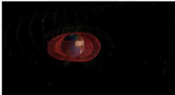
South atlantic anomaly
