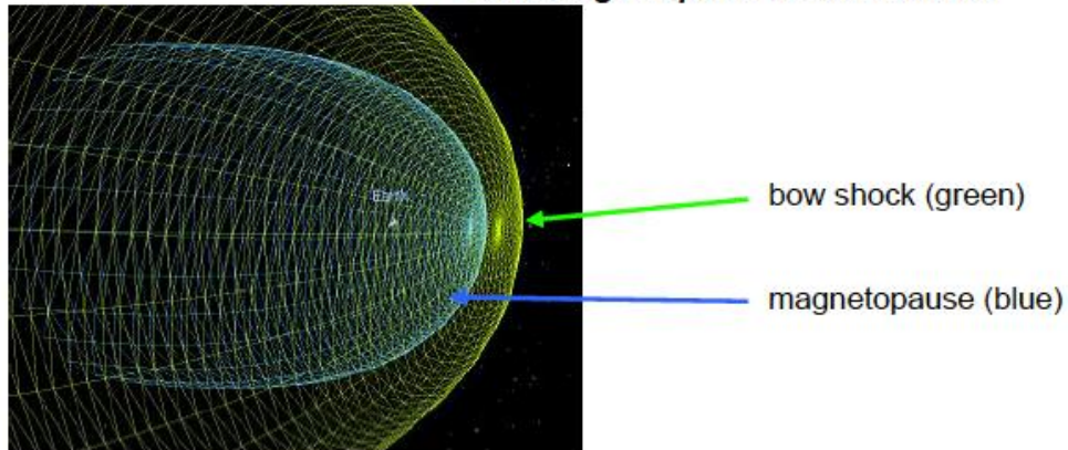
Earth magnetopause and bowshock
